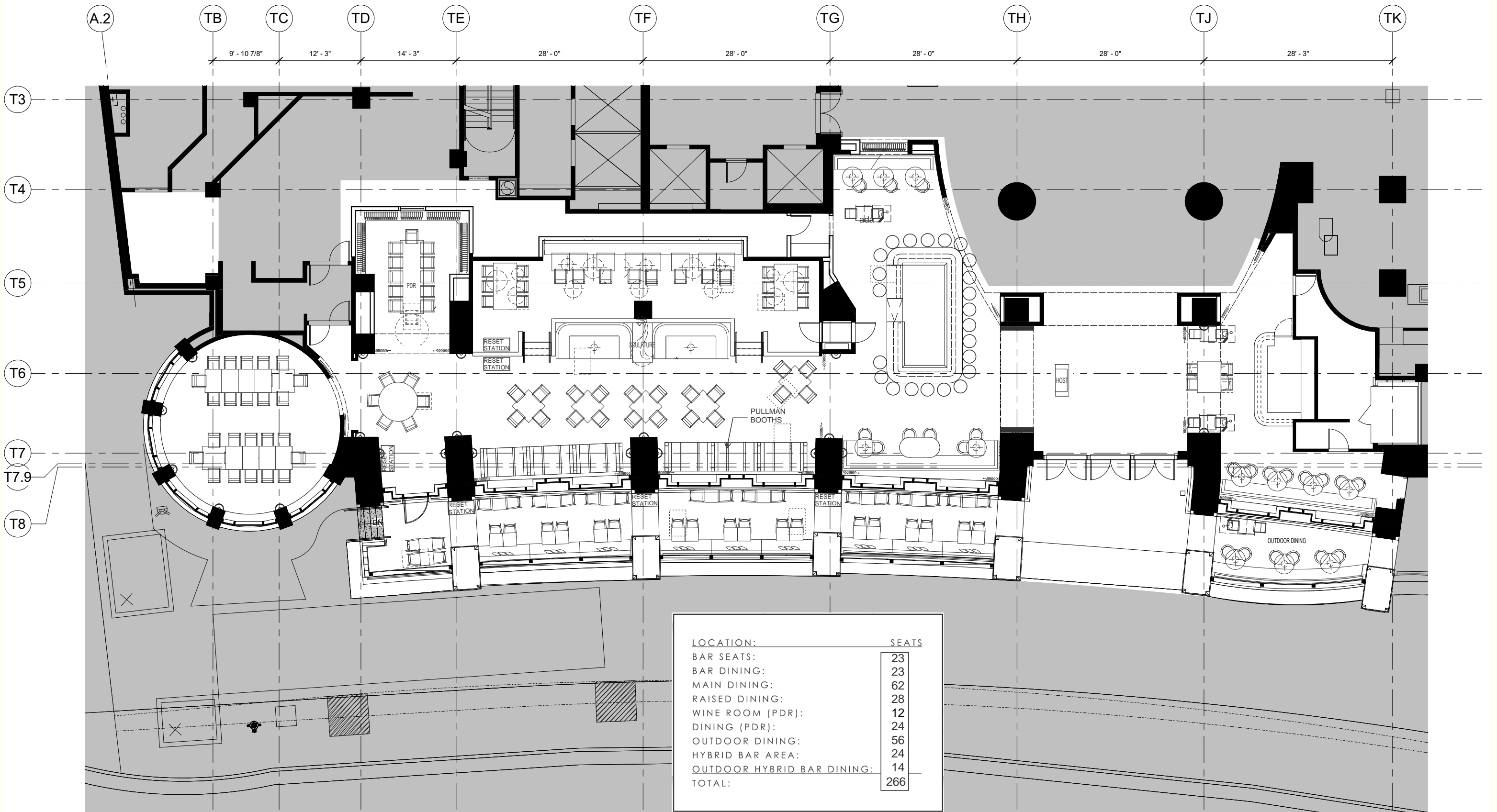
PLAN SKETCH 1
